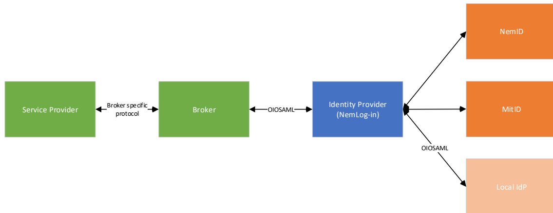
Figure 1: Simple broker integration model
