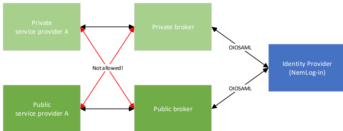
Figur 1: Public and private brokers
