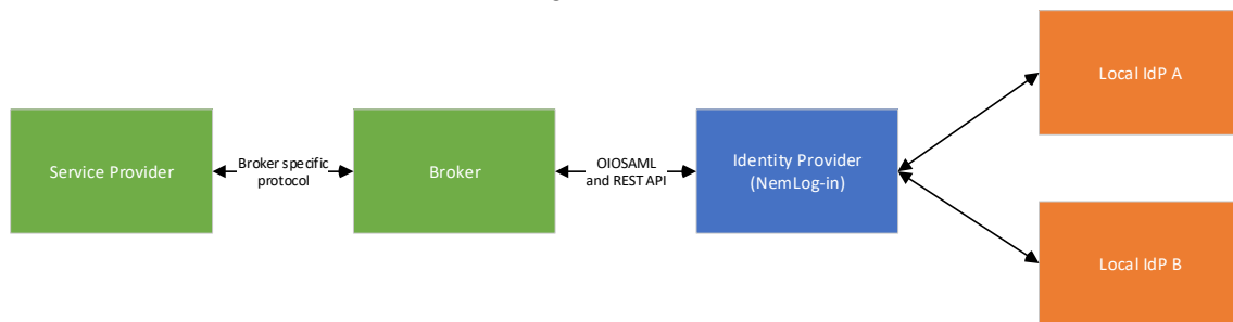
Figure 3: Advanced integration with local IdP
